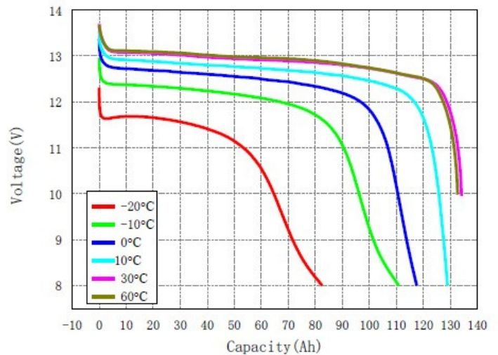
Discharge Curves at Different Temperature
